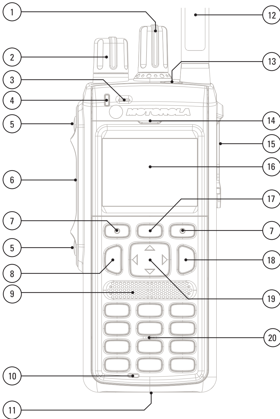
Figure 13: MTP3x50 Series Controls and Indicators
